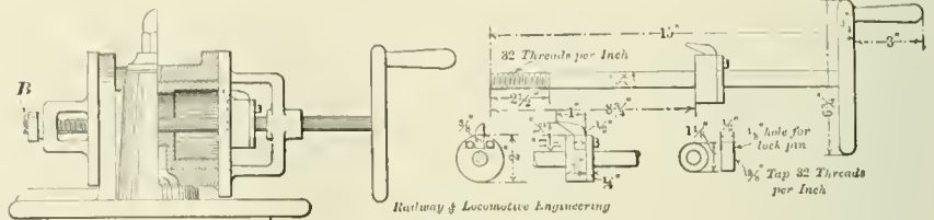
A HANDY TOOL FOR AIR PUMP WORK.
